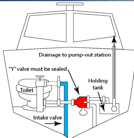
Figure 1: Plumbing connections, such as “Y” valves, can either direct waste into a holding tank, as indicated in the figure above, or overboard. In no discharge zones, the valve must be secured so that it routes waste into a holding tank, rather than into the water.
